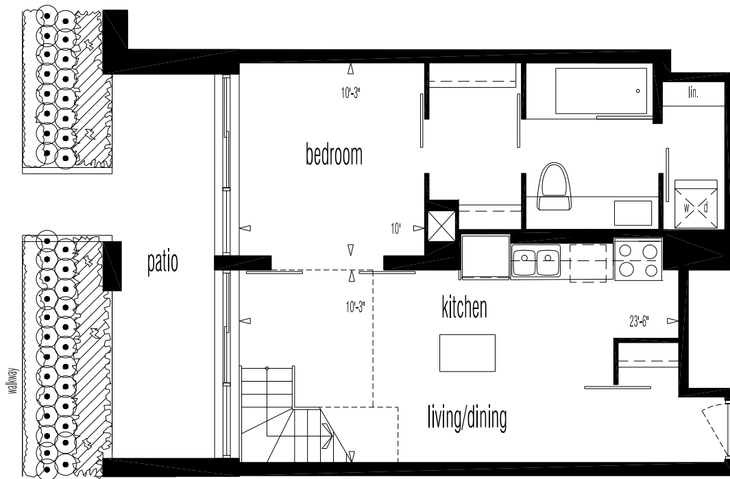
LOWER LEVEL
