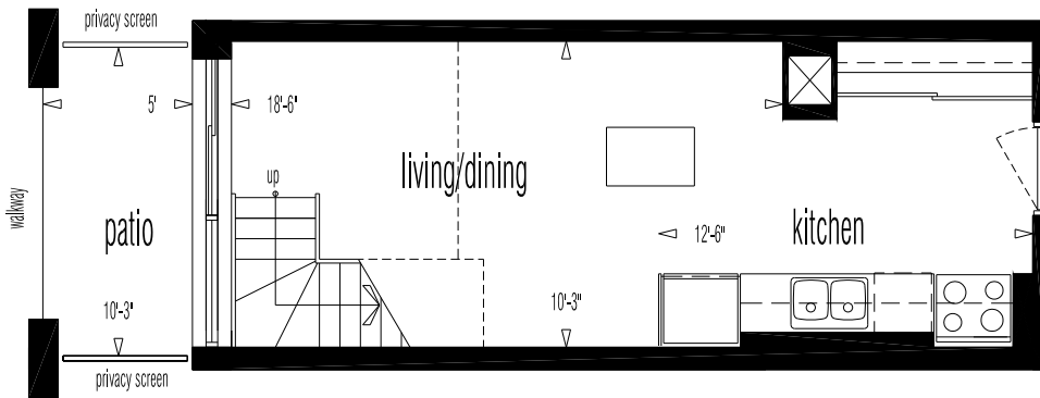
LOWER LEVEL
