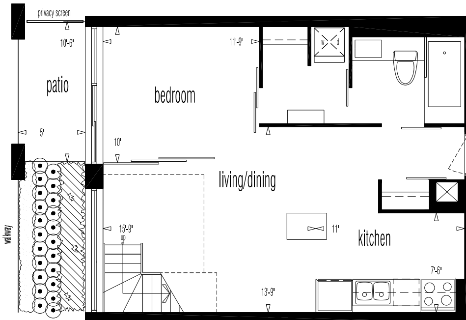
LOWER LEVEL
